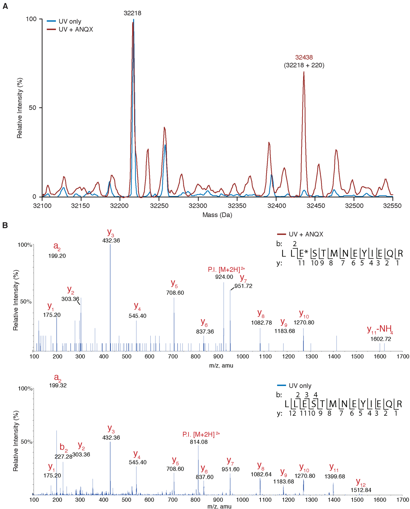
Figure 3. Photocross-linking of ANQX to the GluR2 ligand-binding core (S1S2J) analyzed using mass spectrometry. (A) ESI-o-TOF mass spectrum of the S1S2J (32218 Da) following irradiation (90 s) in the absence (blue trace) and presence (red trace) of ANQX (100 \mu M). Irradiation in the presence of ANQX produces a new major peak (32438 Da) that corresponds to the expected increase in mass (+220 Da) for the ANQX–protein adduct. (B) Mass spectra (MS/MS) of the peptide fragment spanning Glu705 following irradiation (90s) in presence (top panel) and absence (bottom panel) of ANQX. Irradiation in presence of ANQX produced a new peak ( m/z 1602.72, E*, top panel), corresponding to the expected mass increase for the formation of an ANQX adduct, and the loss of unlabeled Glu705 ( m/z 1399.68, E, bottom panel) peak.
